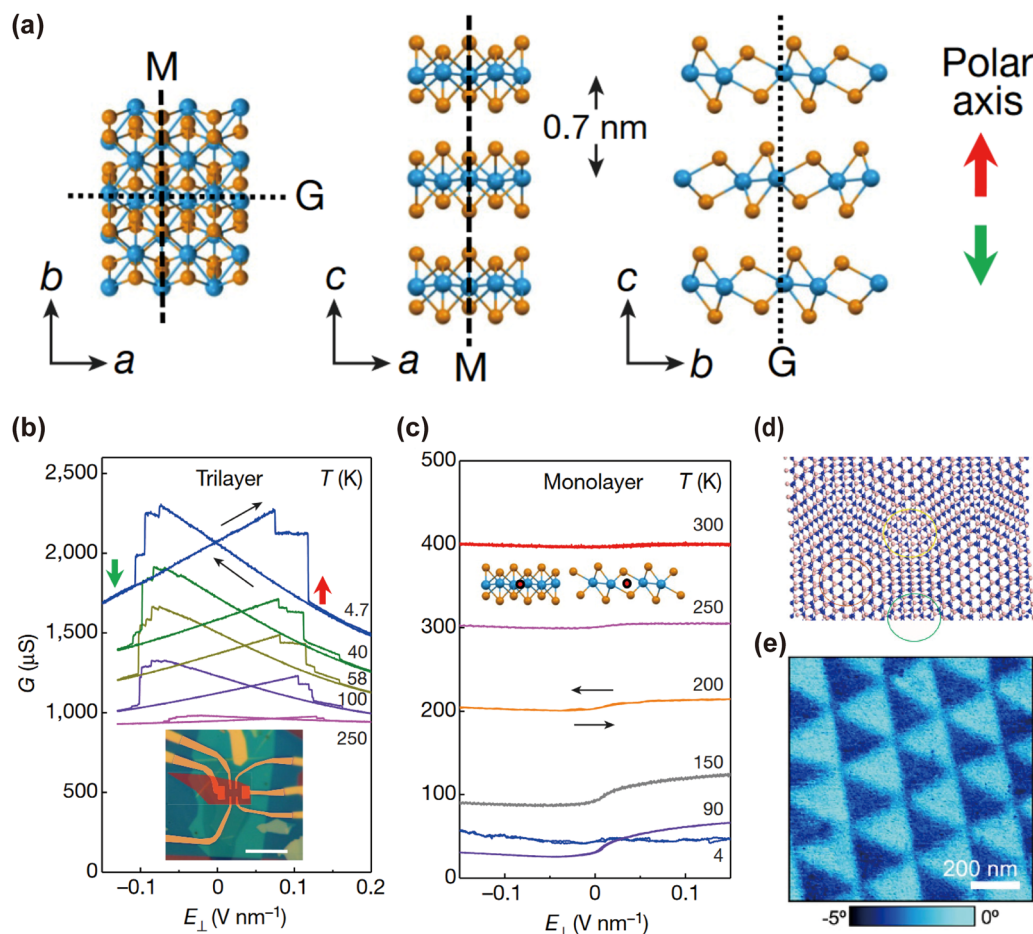
Fig. 10 (a) Top view, side view and front view of the 1T'-WTe 2 homotrimer layer, M represents the mirror plane; G is the sliding plane; red arrow up and green arrow down are polar c-axes. W atoms are in blue; Te atoms are in orange. (b) Conductance G of the undoped trilayer device as E_{\perp} is swept up and down (black arrows). The plots show bi-stability associated with electric polarization up (red arrow) or down (green arrow), at temperatures from 4 K to 300 K (as labelled). Inset is the optical image of a representative double-gated device. (c) Similar measurements on a monolayer 1T'-WTe 2 device (M1), showing no bistability. 173 Reprinted with permission from ref. 173. Copyright 2018, Macmillan Publishers Ltd, part of Springer Nature. (d) Schematic diagram of twisted bilayer h-BN forming moiré superlattice ferroelectricity. 25 Reprinted with permission from ref. 25. Copyright 2017, American Chemical Society. (e) Twisted h-BN ferroelectric domain image with a triangular period. 175 Reprinted with permission from ref. 175. Copyright 2021, The Authors, published by Springer Nature.
