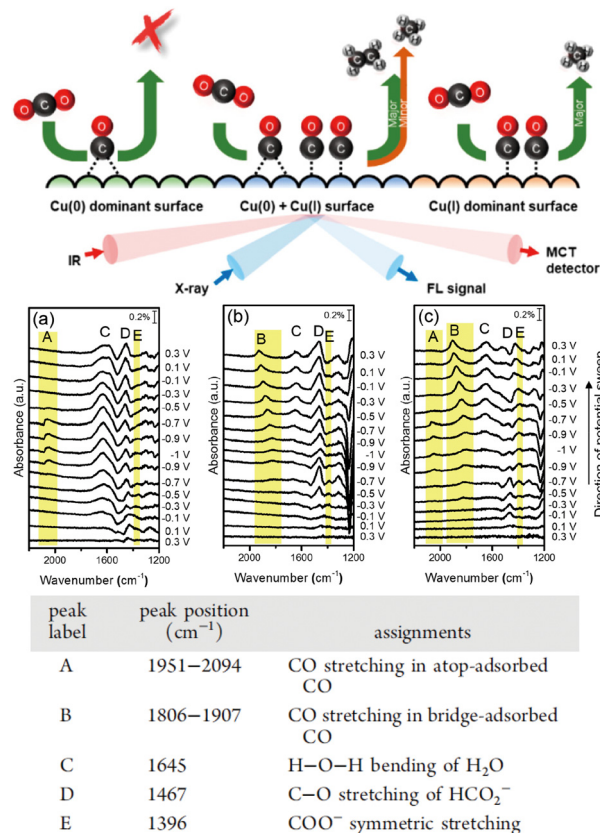
Fig. 4 Upper row: Schematic diagram of the detection of the reaction selectivity and final products on Cu surfaces with different oxidation states using IR and X-ray spectroscopy. Middle row: In situ SEIRAS of the (a) electrodeposited Cu, (b) as-prepared Cu, and (c) CV-treated Cu electrodes during cathodic and anodic scans in \text{CO}_2 -saturated 0.1\text{ mol dm}^{-3}\text{ KHCO}_3 electrolyte solution. Lower row: A table showing the vibrational frequencies and assignments for the species in the IR spectra (a)–(c) under an electrochemical \text{CO}_2\text{RR} . Adapted with permission from ref. 46. Copyright 2020 American Chemical Society. The table shows the vibrational frequencies and assignments for the species in the electrochemical \text{CO}_2\text{RR} . Adapted with permission from ref. 46. Copyright 2020 American Chemical Society.
