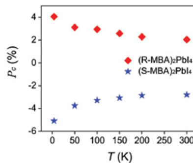
Fig. 8 Temperature-dependent CPL for (R/S-MBA)_2PbI_4 . Reprinted with permission from ref. 27 Copyright©2022 Royal Society of Chemistry.
