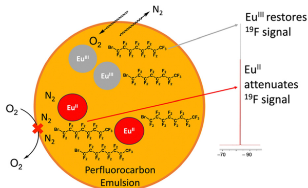
Fig. 5 Cartoon representation of \text{Eu}^{\text{II}}\mathbf{17} in lecithin/perfluorocarbon emulsion. The orange represents a perfluorocarbon mixture surrounding \text{Eu}^{\text{III}}\mathbf{17} , the grey circle, and \text{Eu}^{\text{II}}\mathbf{17} , the red circle.
