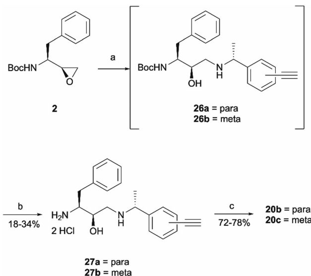
Scheme 6 Synthesis of probes 20b and 20c . Reagents and conditions: (a) Amines 25a/25b , \text{Et}_3\text{N} , \text{MeOH} , 65^\circ\text{C} , o/n; (b) \text{HCl} 4 M in dioxane, DCM, r.t., o/n; (c) 4-benzoylbenzoic acid 21 , HATU, 4-ethylmorpholine, DMSO, r.t., o/n.
