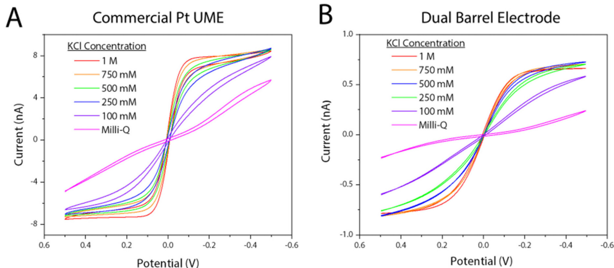
Fig. 6 Changes in voltammetry with changing salt concentration on a (A) commercial CHI platinum UME ( r = 5 \mu\text{m} ) working electrode with a Pt wire quasi-reference counter electrode and (B) a dual barrel electrode (WE r = 0.59 \mu\text{m} , QRCE r = 0.60 \mu\text{m} ). Voltammetry was taken in a 5 mM potassium hexacyanoferrate(II/III) solution with changing salt concentration from 0.5 V to -0.5 V at a scan rate of 0.1 \text{ V s}^{-1} with a 2 seconds quiet time for 5 scans. The final scan for each voltammogram is plotted in polarographic convention.
