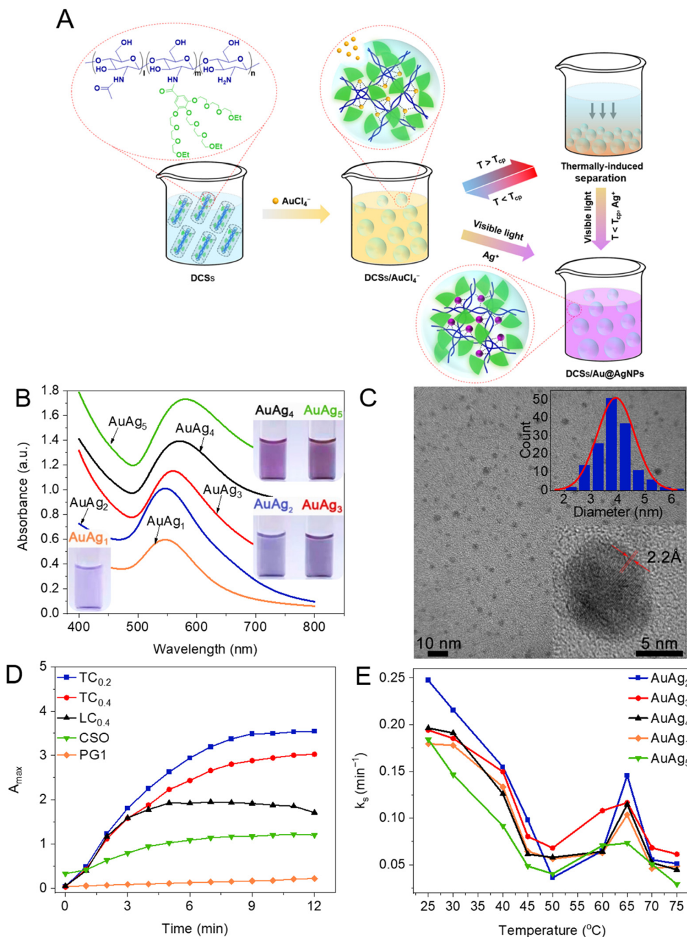
Fig. 6 Fabrication of nanoparticles mediated by DCSs. (A) Schematic illustration of the preparation of Au@AgNPs mediated by DCSs and triggered by visible light. (B) UV-vis spectra of different Au@AgNPs (inset: photographs of the aqueous solutions). (C) TEM image of AgNPs synthesized from DCSs (insets: magnified region and particle size distribution). (D) A_{\text{max}} (at 550 nm) of different Au@AgNPs after shining with visible light for every 1 min interval at 25 °C. (E) The k_s of Au@AgNPs synthesized by DCSs at different temperatures. Reproduced from ref. 34 and 72 with permission from American Chemical Society, copyright 2022.
