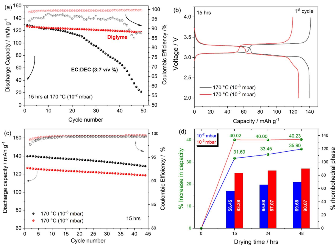
Fig. 8 (a) Cycling behaviour of PW-based electrode dried at 170 °C (10 -2 mbar) in sodium half-cell using 1 M NaPF 6 in EC: DEC (3:7 v/v%) (black curve) and 1 M NaPF 6 in diglyme (red curve). (b) First cycle voltage profiles and (c) corresponding cycling behaviour of PW-based electrodes dried for 15 hours at 170 °C under a dynamic vacuum of 10 -2 mbar (red curve) and 10 -3 mbar (black curve). (d) Comparative data of the percentage increase in capacity relative to the percentage of rhombohedral phase formed upon dehydration at 170 °C for 15, 24, and 48 hours using a dynamic vacuum of 10 -2 and 10 -3 mbar. Tests are conducted at 25 °C within the 2.0–4.0 V range.
