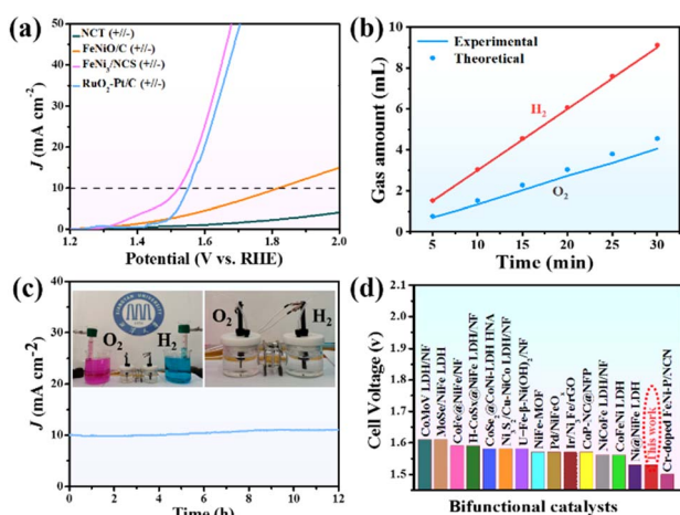
Fig. 7 (a) Overall water-splitting performance of NCT (+||-), FeNiO/C (+||-), FeNi 3 /NCS (+||-), and RuO 2 -Pt/C (+||-) with a scan rate of 5 mV s -1 ; (b) the collected and theoretical H 2 and O 2 volumes at a fixed current density of 10 mA cm -2 ; (c) the long-term durability at a current density of 10 mA cm -2 , and the inset is the photograph of the assembled electrolytic cell; (d) comparison of the overall water-splitting performance of this work and previous reports.
