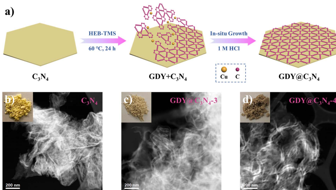
Fig. 1 (a) Schematic illustration for the preparation of GDY@C_3N_4 via a one-pot method. Photographs of samples and corresponding HAADF-STEM images of (b) C_3N_4 , (c) GDY@C_3N_4 -3, (d) GDY@C_3N_4 -4.
