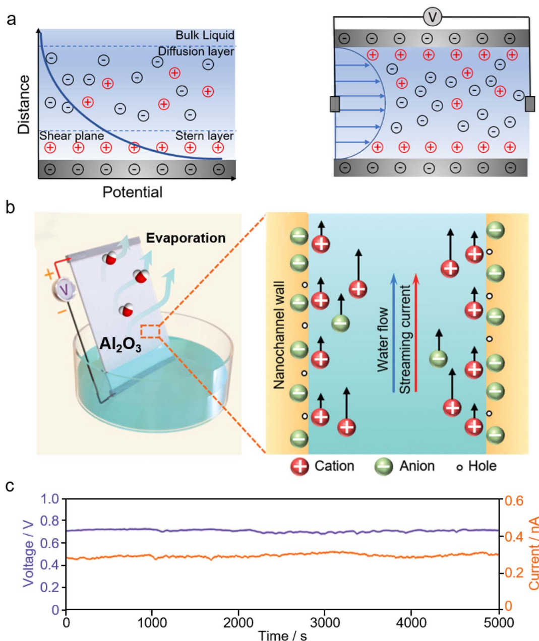
Fig. 8 (a) Schematic illustration of the electric double layer (EDL) formed at the liquid–solid interface (left), and streaming potential generation as a hydrodynamic flow within narrow channels. (b) Schematic illustration of the evaporation-driven electricity generator made from aluminium oxides and (c) its voltage and current output. From, ref. 231 used under the Creative Commons CC-BY license.
