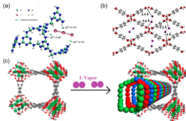
Fig. 7 (a) DFT-calculated hexamer model of MFP bound with I_3^- , the green iso-surface represents strong hydrogen bonding between I and -NH-/-NH_2- . Reproduced with permission from ref. 22. Copyright 2014, Royal Society of Chemistry. (b) Structure of MIL-53(Al) with I_2 adsorbed via hydrogen bonding with the hydroxyl groups. Reproduced with permission from ref. 86. Copyright 2017, American Chemical Society. (c) Schematic of triple-helical chains of iodine molecules formed within the channel of MOF MFM-300(Sc) because of the strong inter-molecular interaction. Reproduced with permission from ref. 88. Copyright 2017, American Chemical Society.
