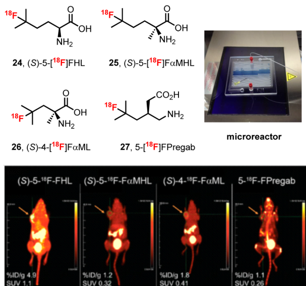
b) Dynamic PET imaging of (S)-5-[ 18 F]FHL (24)
