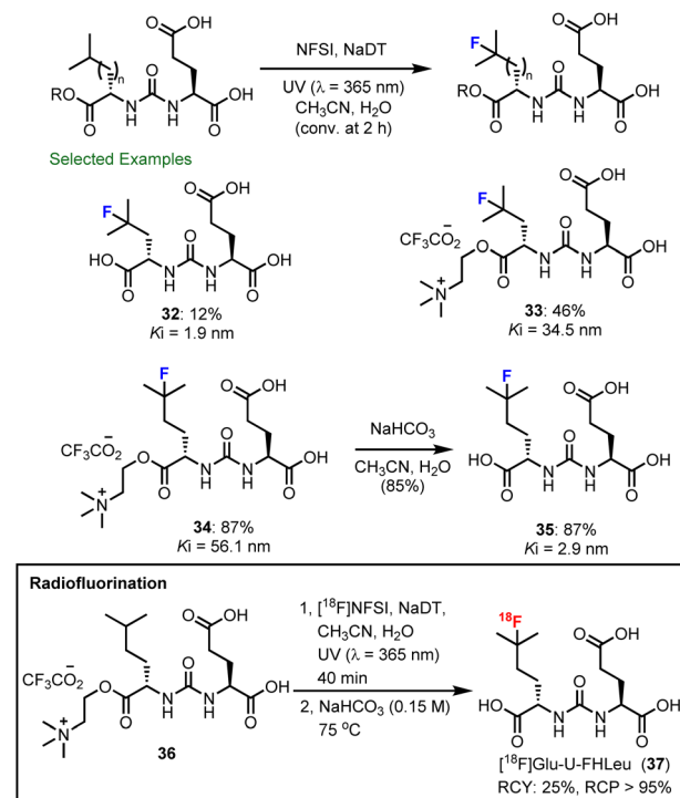
Scheme 9 Accelerated fluorination of choline esters of ZJ-43 and Glu-U-HLeu. PSMA binding of each ligand ( K_i ) was measured by competition assays ( n \geq 3 ) using [ 18 F]DCFPyL and determined by applying a one-site Fit K_i model using GraphPad Prism (7.04).
