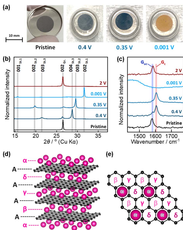
Fig. 3 (a) Photographs of graphite electrodes electrochemically reduced in Rb cells. (b) Ex situ XRD patterns and (c) ex situ Raman spectra of graphite electrodes. (d) Crystal structure model of stage-1 Rb-GIC, \text{RbC}_8 , based on consideration of the in-plane Rb arrangement. (e) Plausible in-plane Rb arrangement in \text{RbC}_8 . The Greek letters from \alpha to \delta represent equivalent Rb positions.
