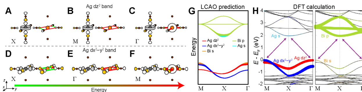
Fig. 8 LCAO analysis for the n = 1 Ag–Bi structure. LCAO representations of the Ag \text{d}_{z^2} derived valence band (VB) at the \text{X} (A), \text{M} (B), and \Gamma (C) points ranked in order of increasing energy from left to right. LCAO representations of the Ag \text{d}_{x^2-y^2} derived VB at the \text{X} (D), \Gamma (E), and \text{M} (F) points ranked in order of increasing energy from left to right. Bonding and antibonding interactions at the \text{B}' site are shown as green and red lines, respectively, and the thickness of each line corresponds to the strength of the interaction. Halide p orbital lobes are scaled to represent approximate relative electron densities and the shading of orbital lobes denote their relative phases. Gray, orange, and brown spheres represent Ag, Bi, and Br atoms, respectively. (G) Predicted band diagram of the n = 1 Ag–Bi structure using our LCAO analysis. (H) DFT band structure of the n = 1 Ag–Bi structure without SOC. The band structure is shown in duplicate where the Ag (left panel) and Bi (right panel) states that compose the bands are represented by colored dots.
