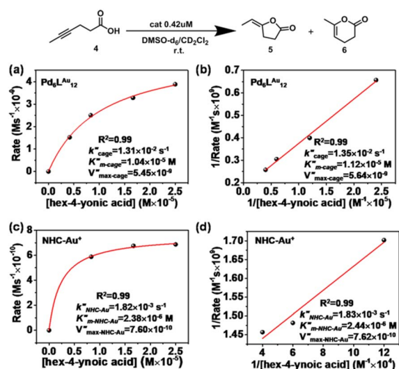
Fig. 7 Kinetic experiments and implications in the cyclization reaction of hex-4-ynoic acid. (a) Kinetic analyses and (b) Lineweaver–Burk plot for the \text{Pd}_6\text{L}^{\text{Au}}_{12} cage. (c) Kinetic analyses and (d) Lineweaver–Burk plot for \text{NHC-Au}^+ .
