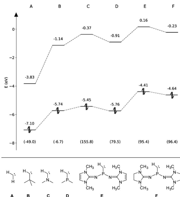
Fig. 4 Eigenenergies of the HOMO and LUMO for carbenes A–F obtained at the B3LYP-GD3BJ/def2-TZVP level. The respective singlet–triplet energy differences ( \Delta E_{\text{ST}} ) are given in kJ mol ^{-1} in parentheses.
