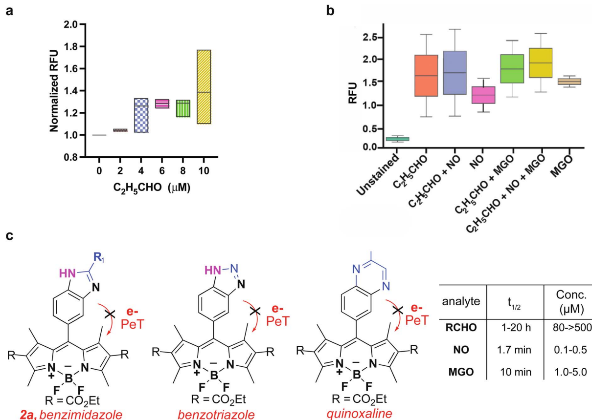
Fig. 4 Detection of aliphatic aldehydes by sensor 1a in live cells. (a) Limit of detection experiments of sensor 1a through incubation of varying concentrations of exogenous propanal (2–10 μM) inside live cells. (b) Selectivity and sensitivity of sensor 1a to image propanal (20 μM) in live cells without interference from NO (0.5 μM) and MGO (5 μM). (c) Sensor 1a product formation upon reactivity with aliphatic aldehydes, NO, or MGO. RFU = relative fluorescence unit. Normalized RFU indicates RFU normalized to sensor 1a . All experiments were performed in triplicate.
