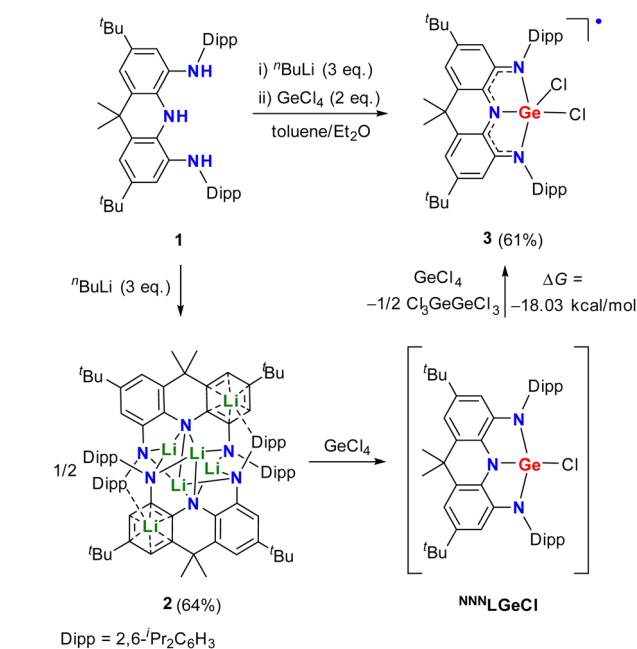
Scheme 1 Synthesis of the germanium precursor 3 .
