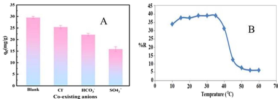
Fig. 9 (A) Effect of co-existing ions on \text{NO}_3^- adsorption onto GCS@LDH. Reproduced with permission from ref. 104 with permission from Elsevier, copyright 2022. (B) The temperature effect on the adsorption of \text{NO}_3^- onto CTS/ZY/ZrO 2 nanocomposite. Reproduced with permission from ref. 87 with permission from Elsevier, copyright 2016.
