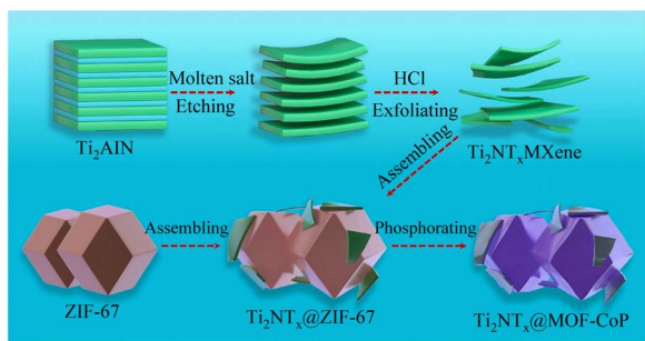
Fig. 13 Schematic of the synthesis of Ti_2NT_x@MOF-CoP . Reproduced from ref. 158 with permission from Elsevier, Copyright 2021.
