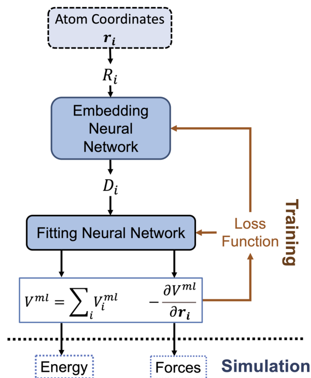
Fig. 1 Workflow for the training of the MLP for implicit solvation of alanine dipeptide. The neural networks are optimized to predict the solute-solute interaction energy V and the corresponding forces on each solute atom.
