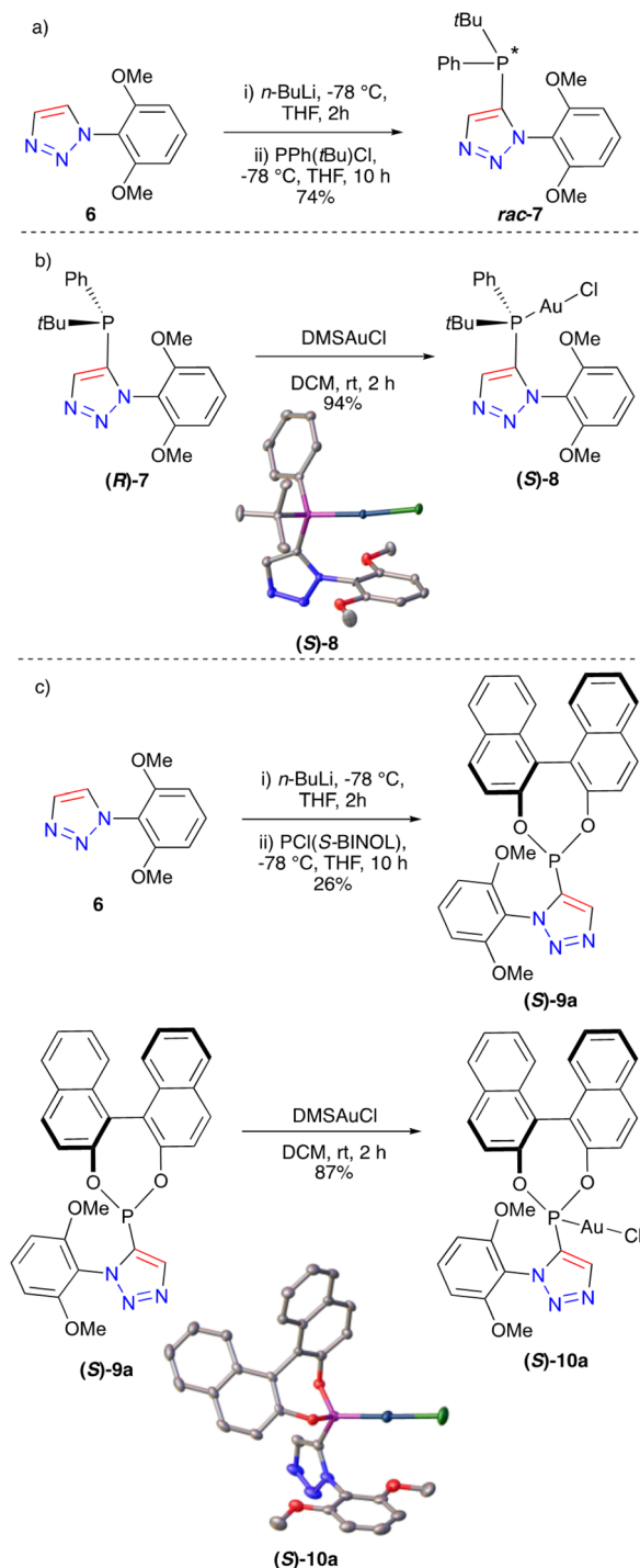
Fig. 4 (a) Synthesis of 1,2,3-triazolephosphine rac - 7 (b) synthesis and single-crystal X-ray diffraction structure of gold(I) chloride complex ( S )- 8 . Ellipsoids are drawn at the 50% probability level (c) Synthesis of 1,2,3-triazole phosphonite ( S )- 9a and subsequent complexation. Single-crystal X-ray diffraction structure of ( S )- 10a . Ellipsoids are drawn at the 50% probability level.
