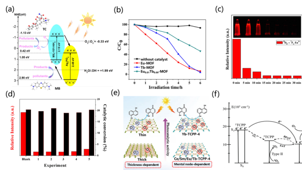
Fig. 5 (a) Schematic of the photodegradation and possible reaction mechanism for the MIL-101-NH 2 /Ag 3 PO 4 system under visible-light irradiation, Copyright 2020, Elsevier. (b) The photocatalytic degradation profiles of RhB under different conditions, Copyright 2019, Elsevier. (c) 5 D 0 → 7 F 2 transition intensity ratios from the emission spectra of MIL-125-AM-Eu introduced into α-phenethyl alcohol after UV radiation for different times. (d) Recycling experiments of MIL-125(Ti)-AM-Eu for sensing α-phenethyl alcohol. Red and black columns represent the luminescence intensity of MIL-125(Ti)-AM-Eu and the conversion of the photocatalytic reaction, respectively, Copyright 2016, American Chemical Society. (e) Illustration of the synthesis of 2D Ln-TCPP nanosheets and the thickness- and metal-node-dependent photocatalytic activity. (f) The possible electron and energy transfer paths in 2D Yb-TCPP-4 nanosheets during the photocatalytic process, Copyright 2020, Wiley VCH.
