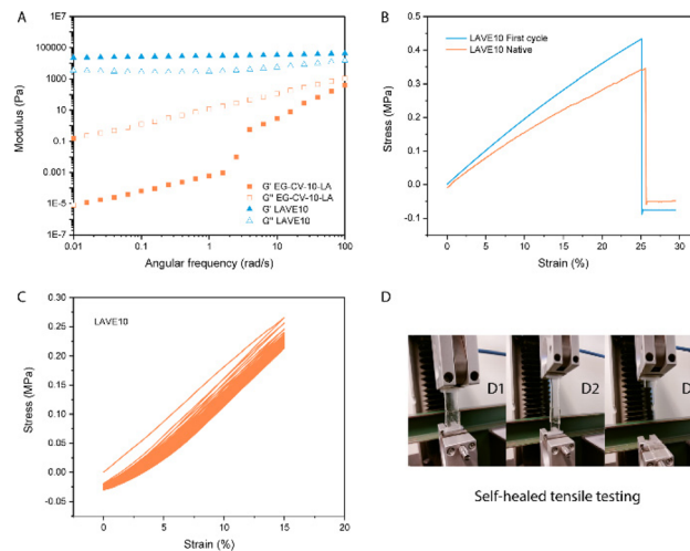
Fig. 4 (A) Oscillatory rheology measurements on EG-CV-10-LA and LAVE10; (B) tensile stress–strain curves of native and first cycle healed LAVE10; (C) cycling test of LAVE10; (D) photograph of healed LAVE30 during tensile testing.
