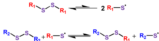
Scheme 1 Radical-mediated dynamic exchange mechanism in disulfides.
