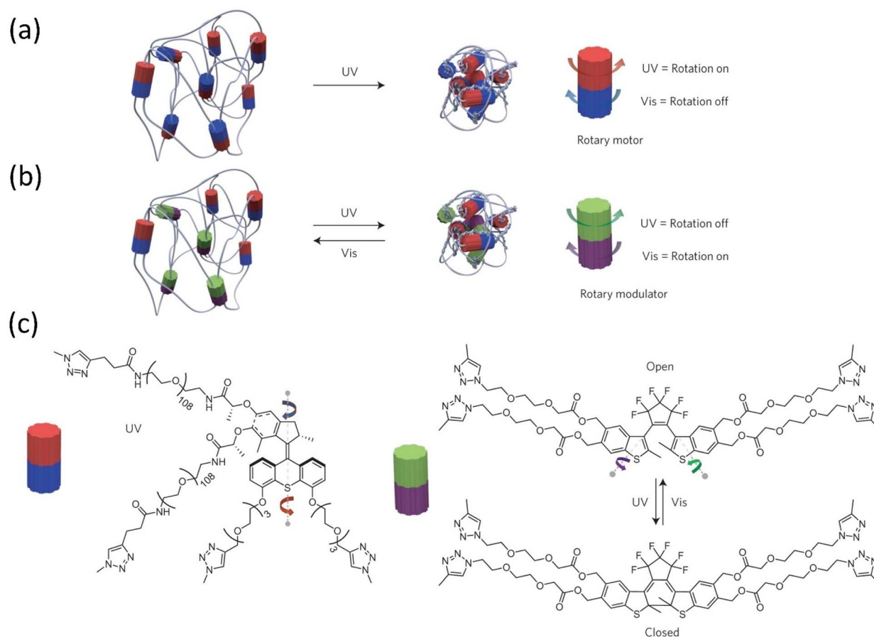
Fig. 19 Dual light control motorized modulator. Graphical representation of (a) a reticulated polymer-motor gel under UV light. (b) A polymer-modulator gel. (c) Dual light control of the polymer-modulator system based on enantiopure overcrowded alkenes rotor and photoswitchable dithienylethenes as the modulators. Reproduced with permission. 120 Copyright 2017, Springer Nature.
