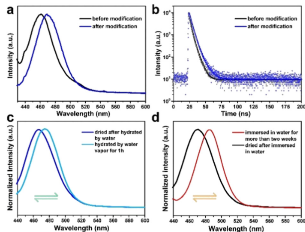
Fig. 5 Water stability of the modified CsPbBr 3 @W-S-1 composite. (a) Fluorescence spectra and (b) fluorescence lifetime decay of the CsPbBr 3 @W-S-1 composite and modified CsPbBr 3 @W-S-1 composite. Reversible PL properties of the modified CsPbBr 3 @W-S-1 composite (c) in water steam and (d) immersed in water.
