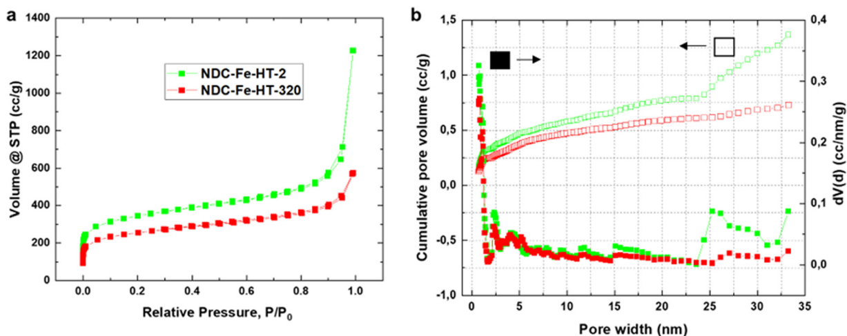
Fig. 3 (a) Isotherms of NDC-Fe-HT-X obtained from \text{N}_2 sorption measurement. (b) The respective pore-size distribution from the adsorption branch employing the QSDFT model for slit and cylindrical pores.
