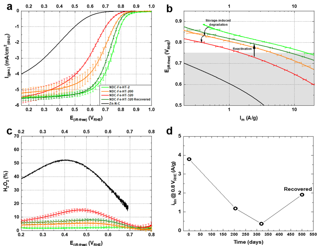
Fig. 2 (a) Capacitance-corrected ORR curves recorded with an RDE setup at room temperature in \text{O}_2 -saturated 0.1 \text{ M HClO}_4 at 1600 \text{ rpm} , 10 \text{ mV s}^{-1} (anodic scans) for NDC-Fe-HT-X and the sample after thermal recovery. The Zn-N-C starting material is plotted to show that the activity of the carbon support starts around 0.75 \text{ V}_{\text{RHE}} . (b) Respective Tafel plots showing purely the kinetic mass activity corrected for mass-transport limitation. The shaded gray area marks the potential region where the support activity takes over. (c) Respective \text{H}_2\text{O}_2 yield obtained via RRDE experiments. (d) Mass activity at 0.80 \text{ V}_{\text{RHE}} of NDC-Fe-HT-X and the sample after thermal recovery.
