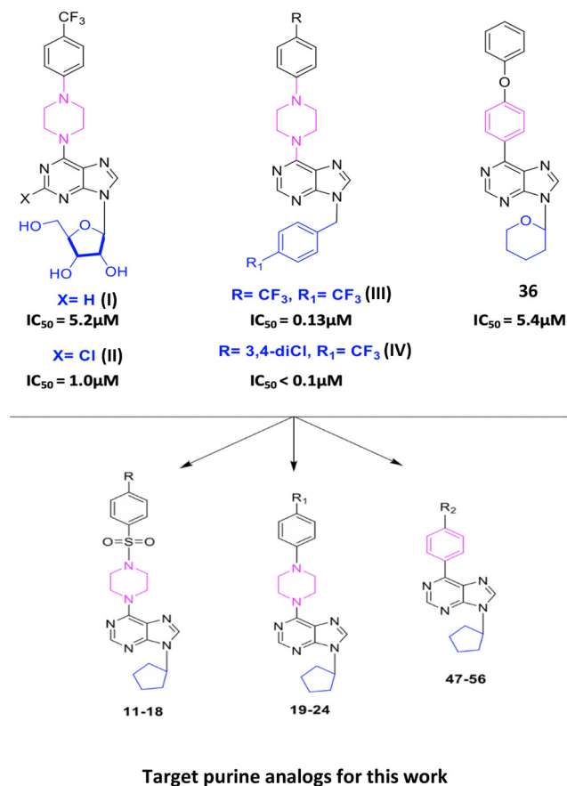
Fig. 1 Structures of 9-( \beta -D-ribofuranosyl)-6-(4-trifluoromethylbenzyl)-4-chlorobenzyl/tetrahydro-pyran)-6-(4-trifluoromethylphenyl)piperazine/4-phenoxyphenyl) purine analogs (I), (II), (III), (IV), and 36 and target purine compounds 11–24 and 47–56.
