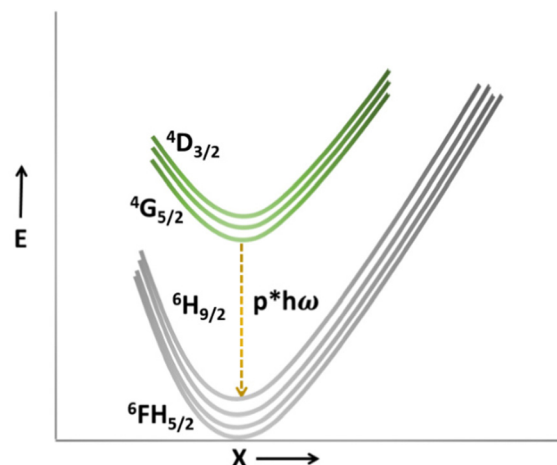
Fig. 9 Schematic model showing thermal quenching of Sm^{3+} .
