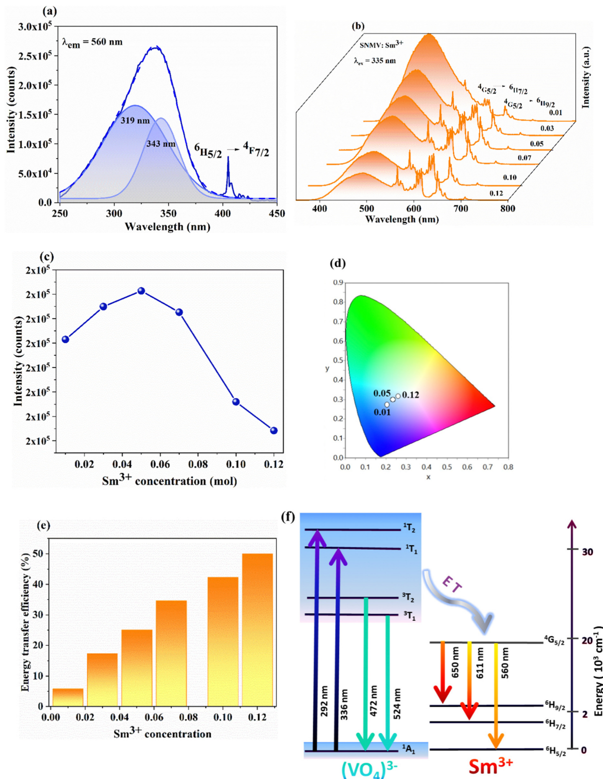
Fig. 4 (a) The PLE spectra monitored under emission at 560 nm, (b) concentration-dependent photoluminescence spectra of SNMV: xSm 3+ ( x = 0.01, 0.03, 0.05, 0.07, 0.10 and 0.12 ) under 335 nm excitation, (c) variation of emission intensity with concentration, (d) CIE diagram of SNMV: 0.01, 0.05 and 0.12 Sm 3+ phosphors, (e) variation of energy transfer efficiency with Sm 3+ concentration, and (f) energy level diagram illustrating the energy transfer from the VO 4 3- complex to Sm 3+ ions.
