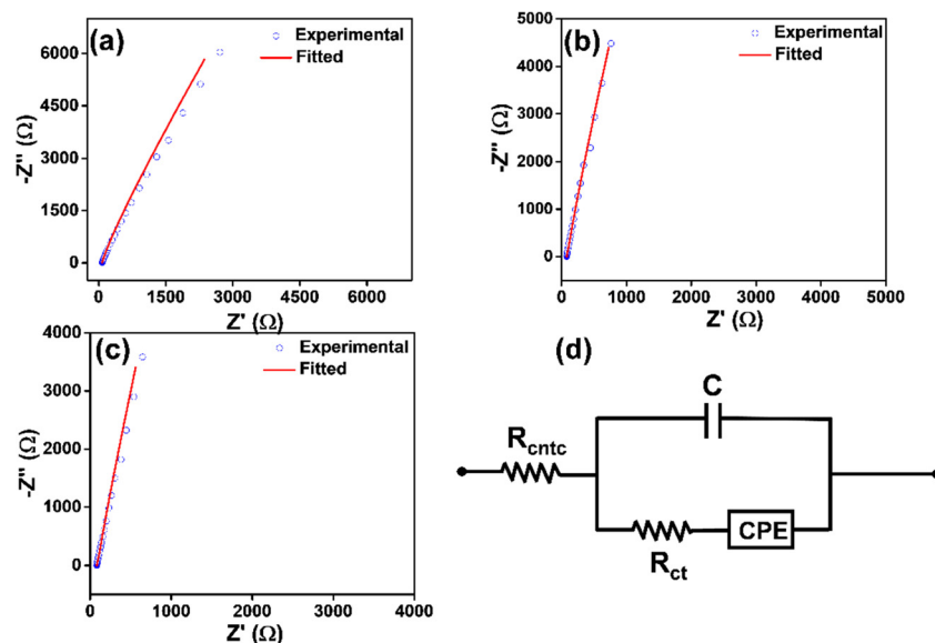
Fig. 7 (a)–(c) Nyquist plots of Ag NPs, L-Cys@Ag, and D-Cys@Ag NPs, respectively and (d) schematic fitted circuit model.
