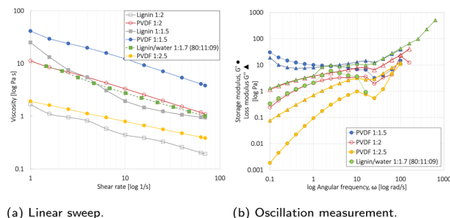
(a) Linear sweep. (b) Oscillation measurement. Fig. 5 Rheology measurement revealing the viscosity for lignin/water or PVDF/NMP based slurries with different powder (NMC111:CB:binder): liquid (P:L) ratios. Unless specified, the powder ratio is 85:10:5 wt% (relative to wt% NMC111). (a) The linear sweep with increasing shear rate from 1–70 1/\text{s} . (b) An oscillation measurement angular frequencies 680–1 \text{rad s}^{-1} revealing the storage modulus ( G' , \bullet ) and loss modulus ( G'' , \Delta ).
