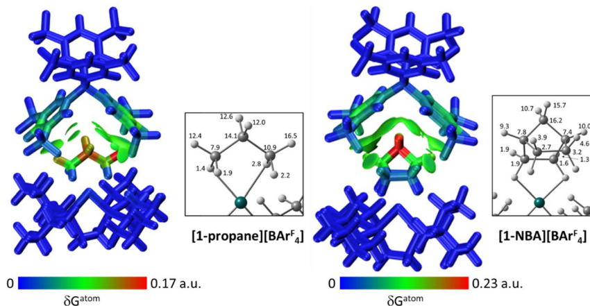
Fig. 6 IGMH plots for the [1-NBA][BAr F 4 ] and [1-propane][BAr F 4 ] top ion-pairs where the cations and anions are defined as separate fragments. Sign( \lambda_2 ) \rho -coloured isosurfaces are plotted with \delta G^{\text{inter}} = 0.003 a.u. and atoms are coloured by % \delta G^{\text{atom}} to highlight their relative contributions. The insets show all % \delta G^{\text{atom}} contributions on the cations that are above 1%.
