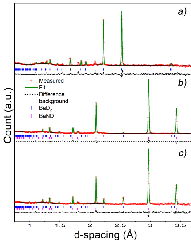
Fig. 9 NPD patterns: (a) starting pattern refined with the HT BaD 2 phase. (b) Pattern 120 (i.e. the middle of the experiment) refined with a HT BaD 2 phase and a BaND phase. The refinement gave an 80% concentration of BaND by weight. (c) Last 73 patterns summed and refined with a BaD 2 and BaND phase. The refinement gave a 96% concentration of BaND by weight.
