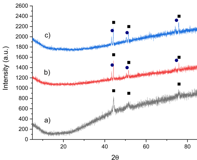
Fig. 6 XRD patterns of \text{Co}_3\text{Cu} : (a) pre \text{N}_2 treatment, (b) post \text{N}_2 treatment at 700 °C and (c) post \text{N}_2 treatment at 800 °C. (■) \text{Co}_3\text{Cu} and (●) Cu.
