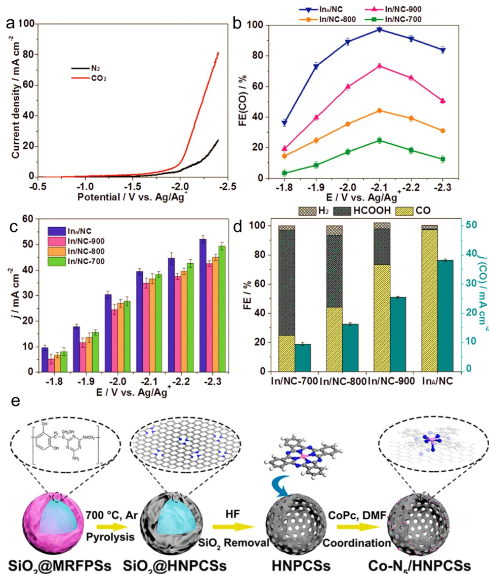
Fig. 26 (a) LSV curves for In A /NC catalyst. (b) FE CO and (c) partial current densities over for CO. (d) FE CO of formate, H 2 and CO. Reproduced with permission from ref. 238 Copyright, 2021 ACS. (e) Schematic of the synthesis of Co-N 5 /HNPCs. Reproduced with permission from ref. 241 Copyright 2018, ACS.
