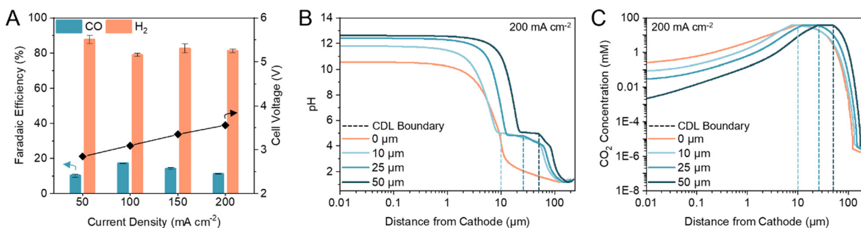
Fig. 2 CDL thickness modulates cathode pH and \text{CO}_2 concentration. (A) FE towards CO and \text{H}_2 in a zero-gap configuration at current densities between 50 to 200 \text{ mA cm}^{-2} . Corresponding full cell voltages are noted on the secondary y-axis. Error bars represent the standard deviation of at least three samples measured under identical conditions. (B) One-dimensional multi-physics modelling of pH at distances from the cathode and current density of 200 \text{ mA cm}^{-2} for CDL with thickness of 0 (zero-gap), 10, 25, and 50 \mu\text{m} . (C) One-dimensional multi-physics modelling of \text{CO}_2 concentration at distances from the cathode and current density of 200 \text{ mA cm}^{-2} for CDL with thickness of 0 (zero-gap), 10, 25, and 50 \mu\text{m} . Accompanying models of \text{HCO}_3^- and \text{CO}_3^{2-} concentrations are provided in the ESI† (Fig. S4).
