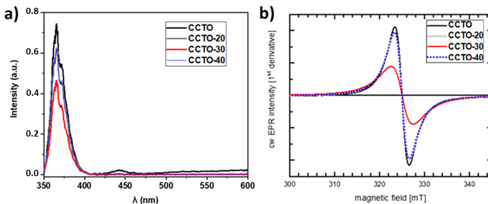
Fig. 5 (a) Photoluminescence spectra and (b) room-temperature cw EPR spectra of the CCTO-20, CCTO-30, CCTO-40 and CCTO samples.
