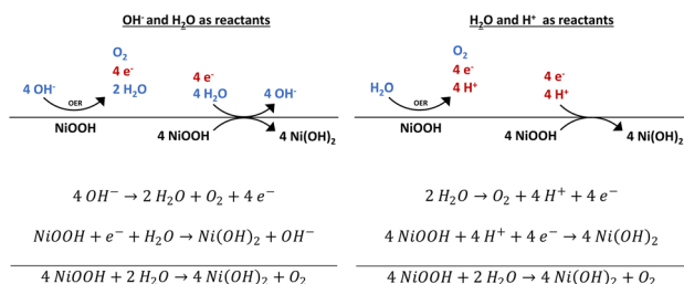
Scheme 1 Decomposition pathways of NiOOH with \text{H}_2\text{O} and \text{OH}^- or \text{H}^+ as reactants. NiOOH catalyses the oxygen evolution reaction (OER), which provides the electrons for the \text{Ni}^{3+} to \text{Ni}^{2+} reduction. The protons for the phase transformation of NiOOH to \text{Ni(OH)}_2 are either delivered by the OER pathway as well or by the dissociation of \text{H}_2\text{O} molecules.
