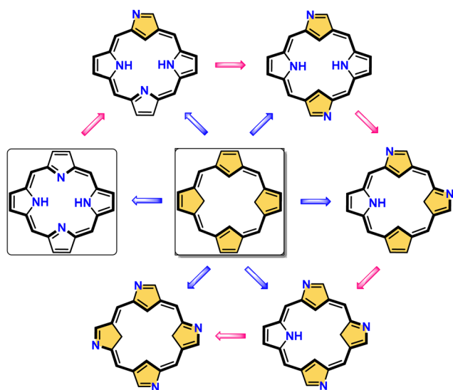
Scheme 133 Complementary strategies: inner core/perimeter four nitrogen atom nitriding of quaternary (blue arrows) and stepwise N-confusion of regular porphyrin (blue arrow nitriding and purple arrow N-confusion).
