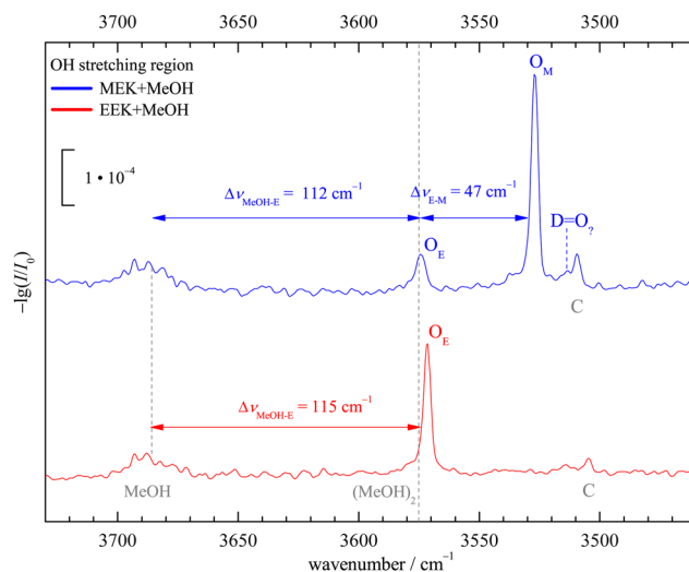
Fig. 4 Jet FTIR OH-stretching spectra of MeOH in co-expansion with MEK and EEK including the MeOH monomer region. C marks a non 1 : 1 stoichiometry and D=O₂ is the largest isolated signal which might perhaps be attributed to a third 1 : 1 isomer in the MEK case, beyond the dominant O M (M docking) and the secondary signal O E (sE docking, common to both ketones). For details, see the main text.
