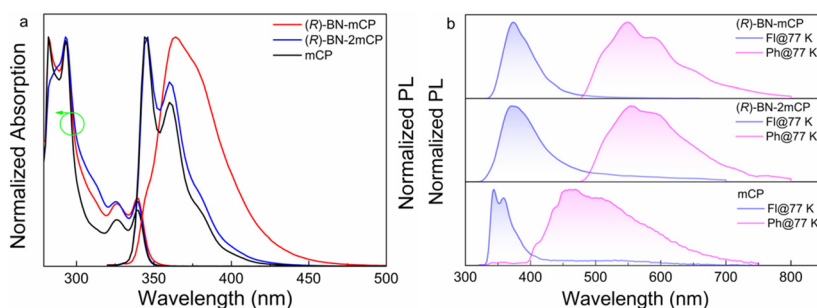
Fig. 2 (a) UV-vis spectra and PL spectra ( \lambda_{ex} = 300 nm) measured in toluene solution ( 10^{-5} M); (b) fluorescence and phosphorescence in the doped PMMA film (10%) at 77 K temperature ( \lambda_{ex} = 300 nm).
