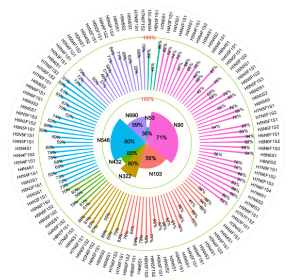
Fig. 4 The distribution of α2,3-sialylation on N -glycopeptides and specific glycosites of hACE2. The contents of α2,3-linked sialic acid isomer of glycans on specific N -glycosites are labeled in the outer circle, corresponding to the glycan compositions. The overall proportions of α2,3-sialylation presented on specific N -glycosites are illustrated in the inner circle. N53, N90, N103, N322, N432, N546 and N690 are colored green, pink, carmine, toast tan, grass green, blue, and purple, respectively.
