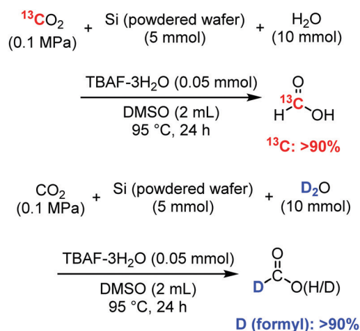
Scheme 1 Isotopic experiment. ^{13}\text{C}\text{O}_2 : powdered silicon wafer (5 mmol; diameter < 20\ \mu\text{m} ), ^{13}\text{C}\text{O}_2 (1 atm), \text{H}_2\text{O} (10 mmol), TBAF- 3\text{H}_2\text{O} (0.05 mmol), DMSO (2 mL), 95\ ^\circ\text{C} , 24 h. \text{D}_2\text{O} : powdered silicon wafer (5 mmol; diameter < 20\ \mu\text{m} ), \text{CO}_2 (1 atm, balloon), \text{D}_2\text{O} (10 mmol), TBAF- 3\text{H}_2\text{O} (0.05 mmol), DMSO (2 mL), 95\ ^\circ\text{C} , 24 h.
