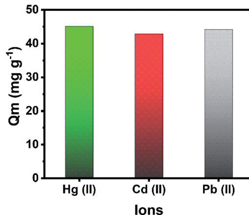
Fig. 5 Simultaneous removal of \text{Hg(II)} , \text{Cd(II)} , and \text{Pb(II)} from a ternary metal solution. Conditions: mass of \text{Zr-MOF@Fe}_3\text{O}_4 = 30 \text{ mg} , [\text{ion}] = 50 \text{ mg L}^{-1} each, volume = 30 mL, time = 12 h.
