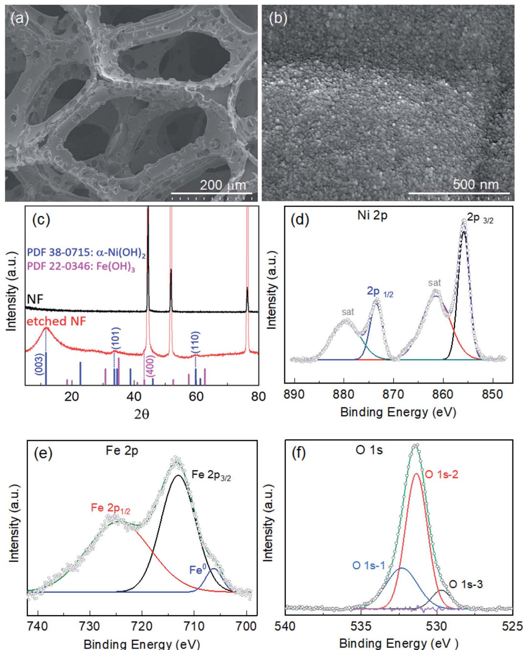
Fig. 1 SEM images of nickel foam (NF) etched for 18 h (Fe-18h/NF) in an ethanolic \text{FeCl}_3 solution at 50 °C: (a) surface view showing microporous Ni backbones at low magnification, and (b) a high-magnification view showing hierarchically-structured metallic Fe@Ni-Fe-hydroxide nanoparticles with a diameter of \sim 10 nm. (c) XRD patterns of pristine NF and NF etched for 18 h. XPS spectra of (d) Ni 2p, (e) Fe 2p, and (f) O 1s for the Fe-18h/NF sample.
