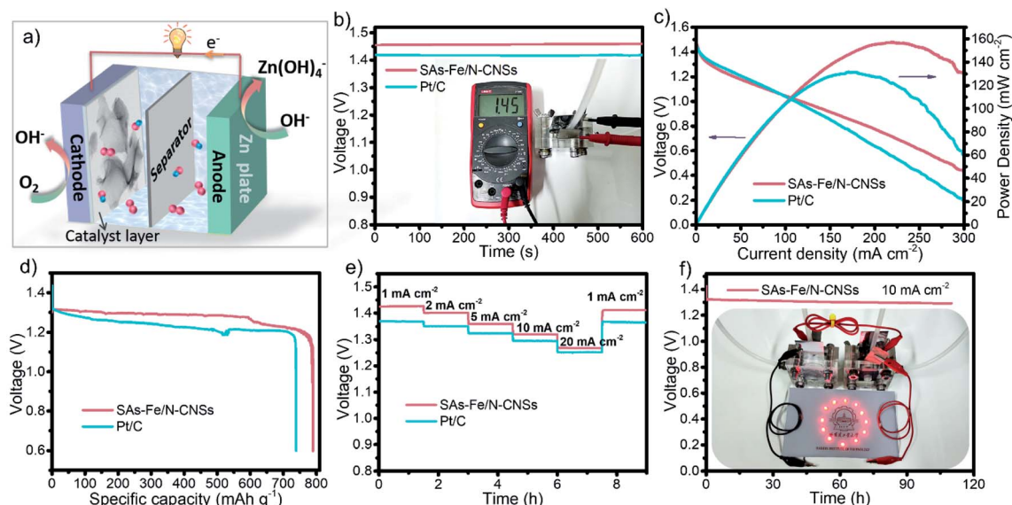
Fig. 5 (a) Schematic drawing of the primary Zn-air battery ( \bullet : OH^- , \bullet : O_2 ). (b) Open-circuit voltage result of SAs-Fe/N-CNSs and Pt/C. (The inset exhibits the photograph for the open-circuit voltage of the SAs-Fe/N-CNSs-based battery performed using a multimeter.) (c) Polarization together with power density curves towards SAs-Fe/N-CNSs- and Pt/C-assembled Zn-air batteries. (d) Specific capacity result at 10\ mA\ cm^{-2} towards batteries utilizing SAs-Fe/N-CNSs and Pt/C as cathode materials (standardized with the mass of consumed Zn). (e) Rate capability of batteries utilizing SAs-Fe/N-CNSs and Pt/C as cathode materials. (f) Stability measurement at 10\ mA\ cm^{-2} for batteries utilizing SAs-Fe/N-CNSs as cathode materials (recharged via renewing electrolyte circularly). (The inset is the photograph of red LEDs lightened through two Fe/N-CNSs Zn-air batteries in series.)
