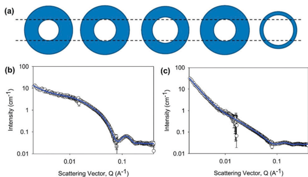
Fig. 12 (a) Cartoon representation of hollow cylinder cross-sections obtained from the fitting of SANS data for (from left to right) 2NapFF, 2dNapFF, 2NapdFdF, 2NapdFhF and 2NapdFf. SANS data for (b) 2dNapFF in D 2 O (second from left in cartoon) and (c) 2NapdFdF in D 2 O (far right in cartoon). Reproduced from E. R. Draper, B. Dietrich, K. McAulay, C. Brasnett, H. Abdizadeh, I. Patmanidis, S. J. Marrink, H. Su, H. Cui, R. Schweins, A. Seddon, D. J. Adams, Matter , 2020, 2 , 3, 764–778, with permission from Elsevier (Copyright © 2020) under the Creative Commons CC-BY (version 4.0) license.
