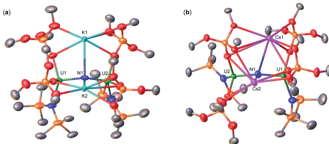
Fig. 4 Molecular structures of (a) [K_2\{U^{IV/III}(\text{OSi}(\text{O}^t\text{Bu})_3)_2(\text{N}(\text{SiMe}_3)_2)_2(\mu\text{-N})\}] , 6-K , and (b) [Cs_2\{U^{III/IV}(\text{OSi}(\text{O}^t\text{Bu})_3)_2(\text{N}(\text{SiMe}_3)_2)_2(\mu\text{-N})\}] , 6-Cs , with thermal ellipsoids at drawn at the 50% probability level. Hydrogen atoms and methyl groups on the \text{OSi}(\text{O}^t\text{Bu})_3 ligands have been omitted for clarity.
